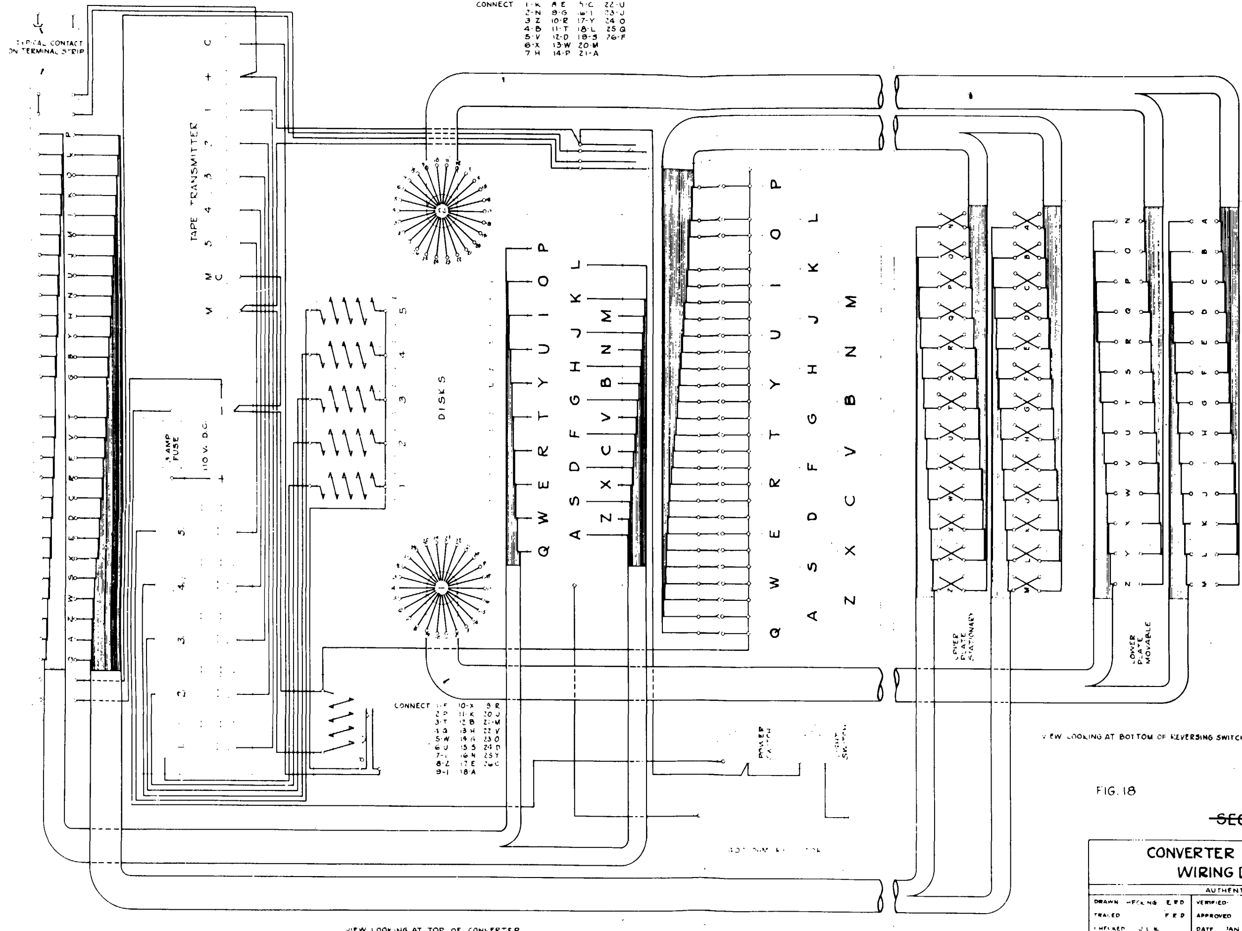
VIEW LOOKING AT TOP OF CONVERTER
