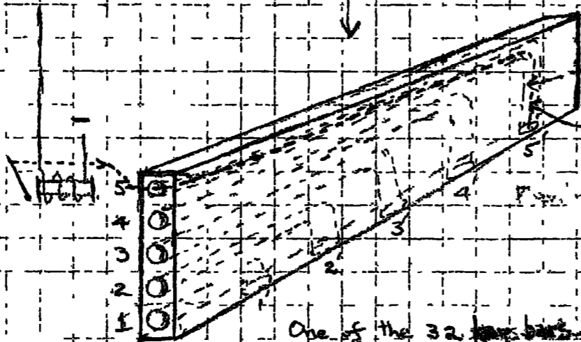
Tube through which flexible rod or Dowdoin wire pushes out "projection". Magnet at left supplies motive power.
